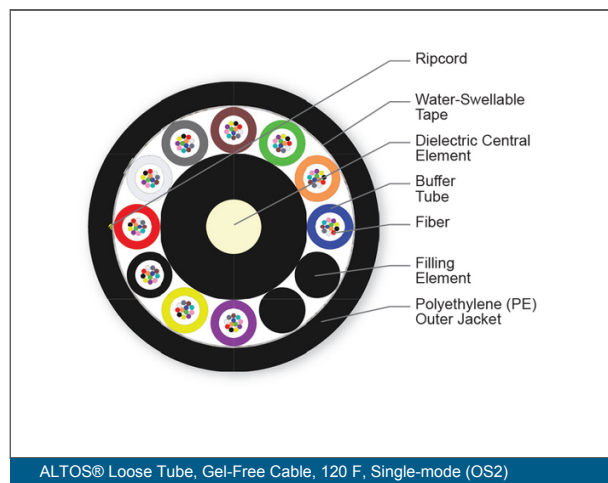
ALTOS® Loose Tube, Gel-Free Cable, 120 F, Single-mode (OS2)
